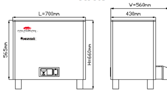
OCS-180B
